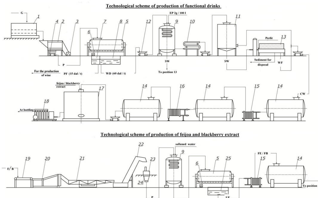
Fig.4. Technological scheme of production of functional drinks based on grape juice
